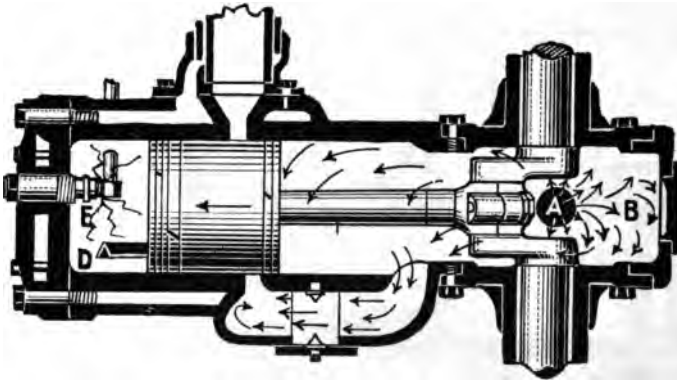
FIG. 130.—Diagram of the Two-part Cycle of a Gas Engine, I. The instroke of the piston, showing the aspiration of fuel gas at A, into crank case, B, and the spark at E in combustion space, D.
